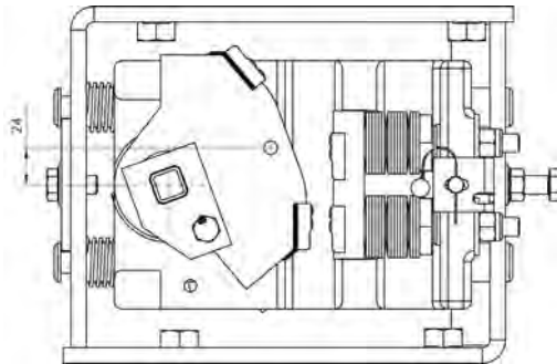
Pict. 1: Distance of application for safety gear actuated directly at rotary disc
